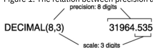
Figure 1. The relation between precision and scale in a fixed-point number
